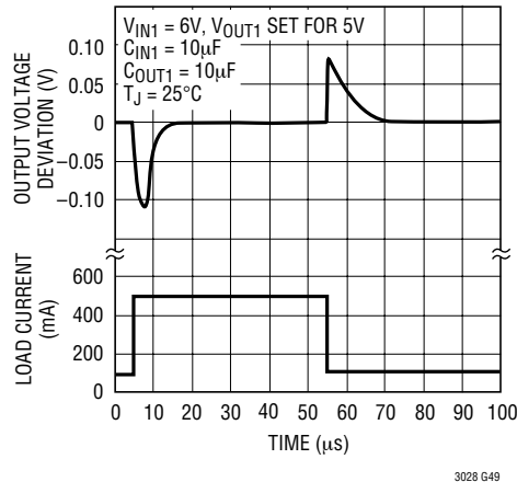
Output 1 Transient Response C_{BYP} = 0.01µF
