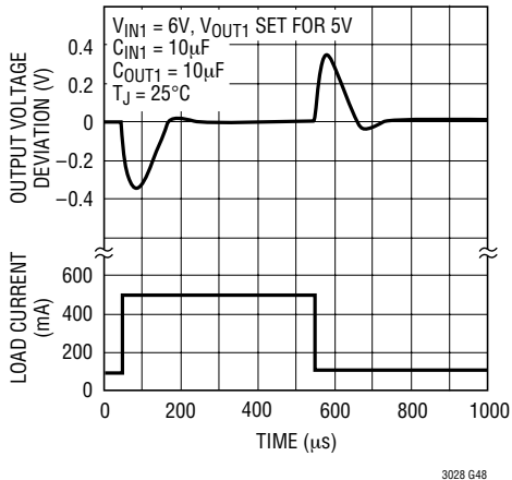
Output 1 Transient Response C_{BYP} = 0pF
