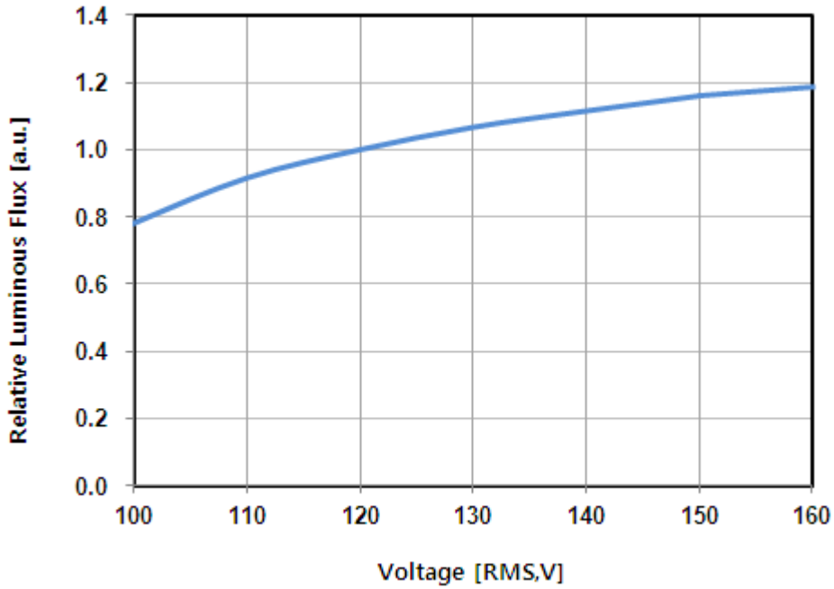
Fig 6. Relative Luminous Flux vs. Voltage at T_a=25^{\circ}\text{C} , 220V
