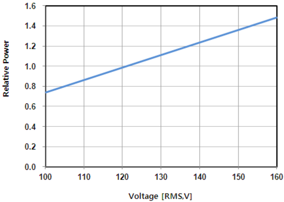
Fig 4. Relative Power Distribution vs. Voltage at T_a=25^{\circ}\text{C} , 120V
