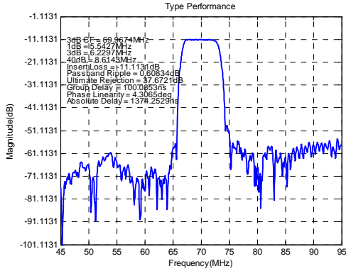
Frequency Respond
