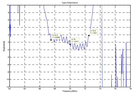
Phase Linearity (f0±2.5MHz)
