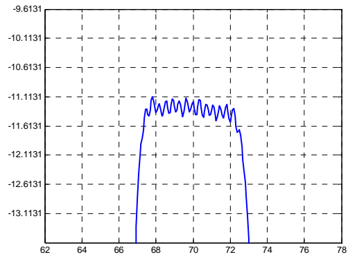
Passband Respond
