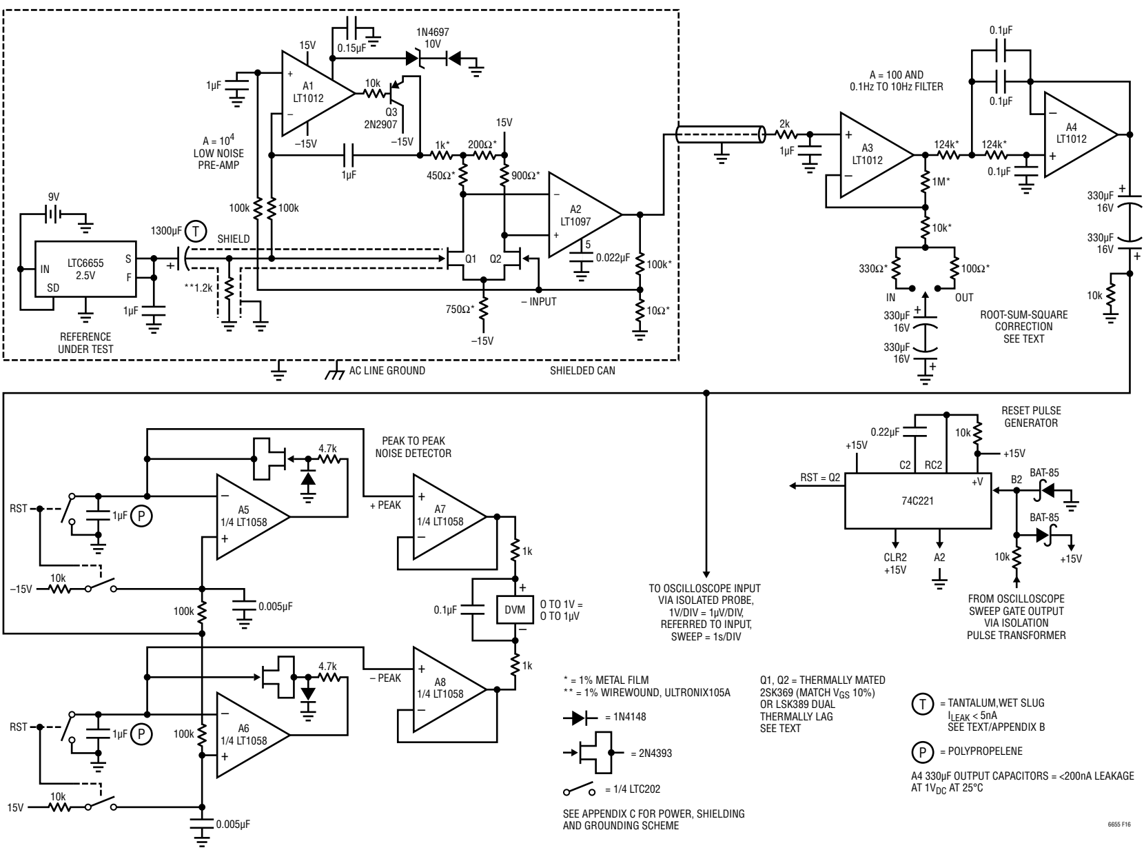
Figure 17. Detailed Noise Test Circuitry. See Application Note 124.
