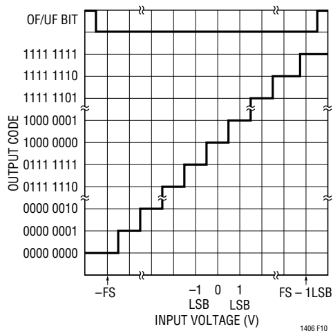
Figure 10. Transfer Characteristics
