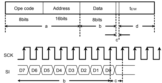
Figure 41. WRITE cancel valid timing
