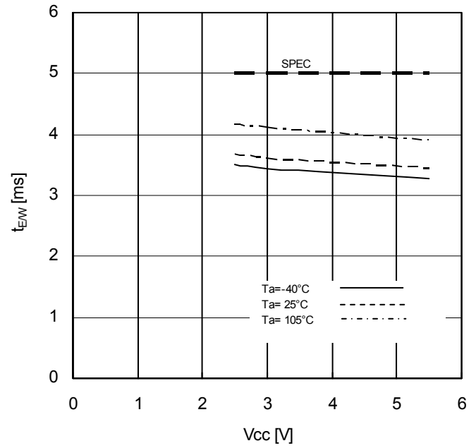
Figure 31. Write Cycle Time vs Supply Voltage
