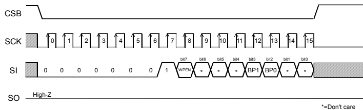
Figure 36. Write status register
