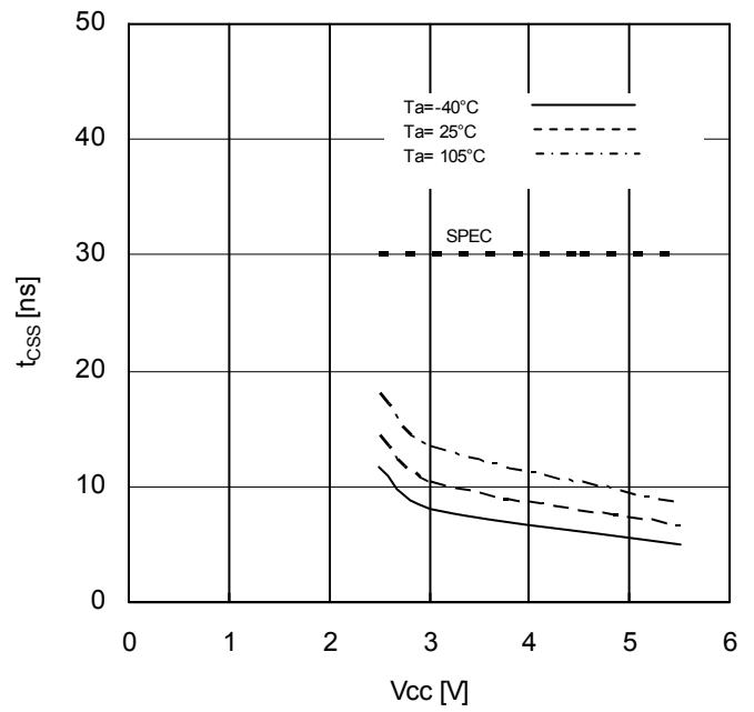
Figure 19. CSB Setup Time vs Supply Voltage
