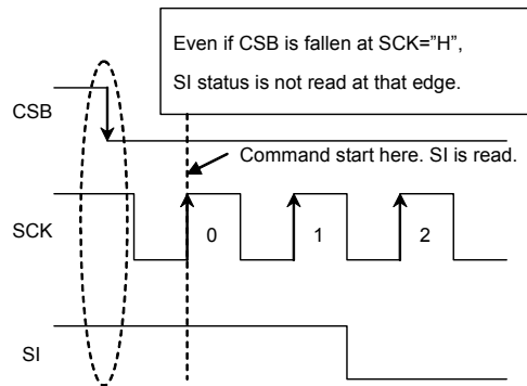
Figure 54. Operating timing
