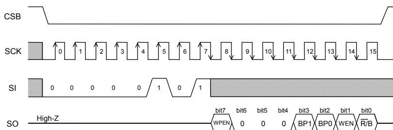
Figure 37. Read status register command
