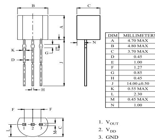
TO-92
