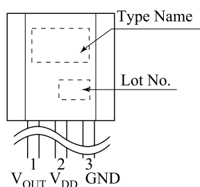
TO-92
