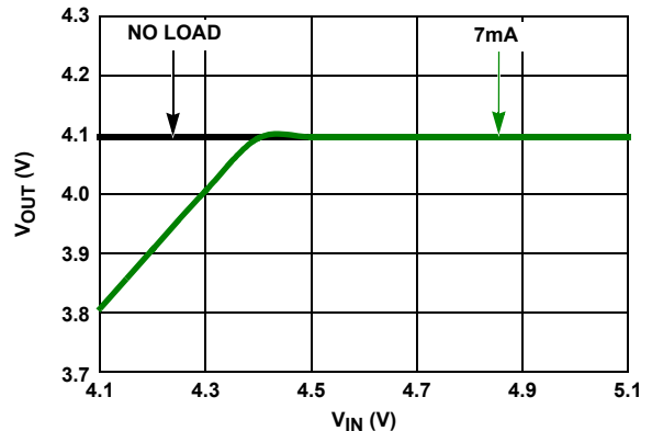
FIGURE 33. DROPOUT, ISL21080-41
