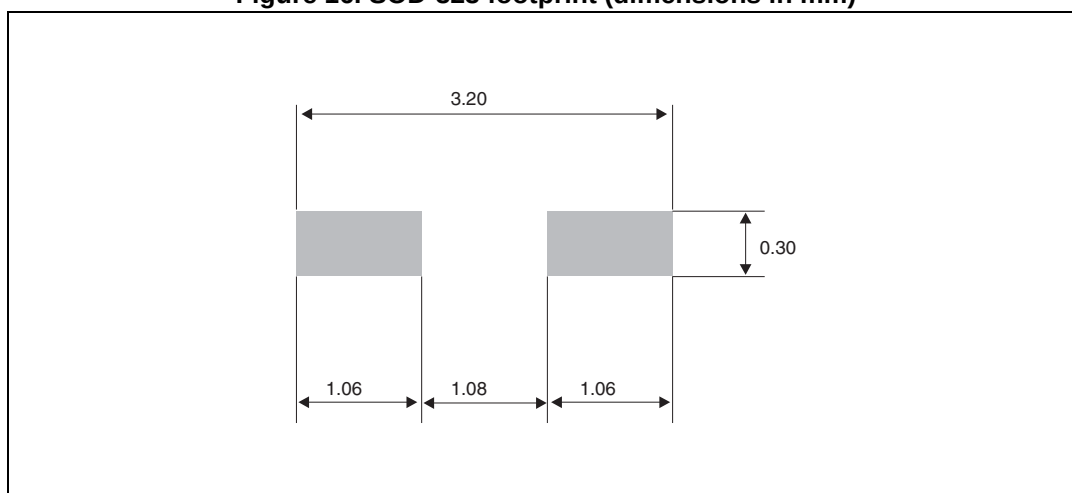
Figure 16. SOD-323 footprint (dimensions in mm)
