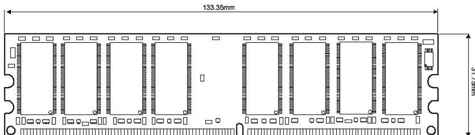
Figure: mechanical dimensions
