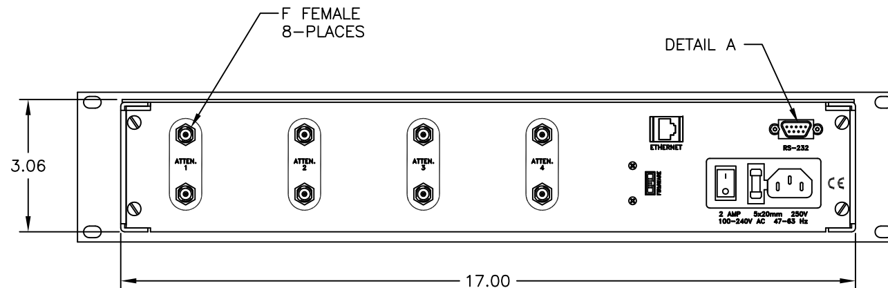
REAR VIEW
