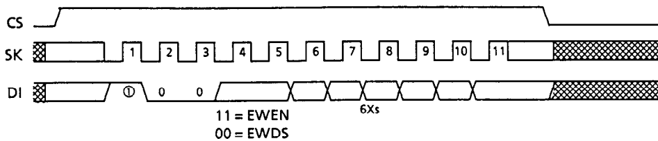
Figure 15 EWEN/EWDS Timing (S-29U331A)
