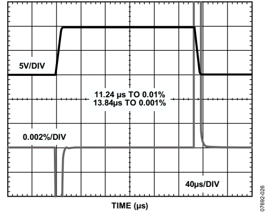
Figure 28. Large-Signal Pulse Response and Settling Time, 10 V Step, V_S = \pm 15\text{ V}
