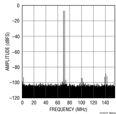
LTC2153-12 32K Point 2-Tone FFT, f IN = 71MHz and 69MHz, 310Mps
