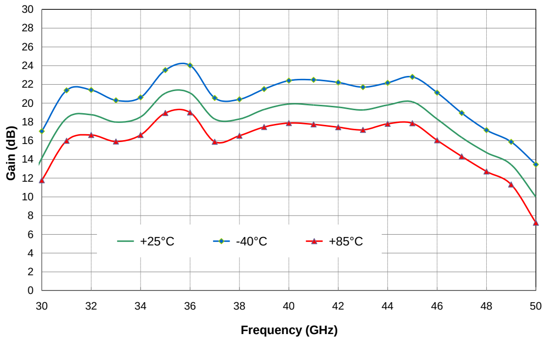
Gain versus frequency &amp; temperature
