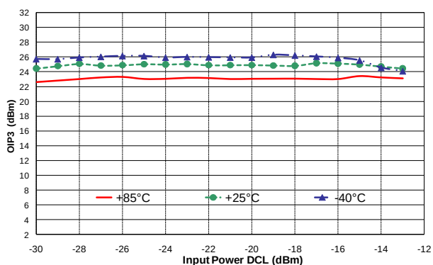
Output IP3 versus temperature at 120mA & 40GHz
