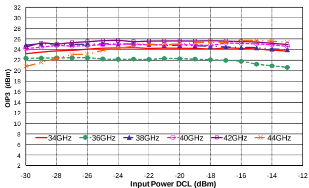
Output IP3 versus frequency at 120mA
