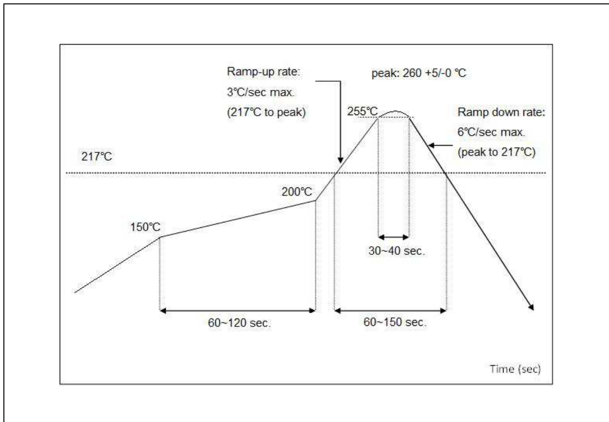
FIGURE 7-1: REFLOW PROFILE
