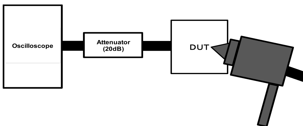
Fig. 10.3 IEC61000-4-2 (Contact)
