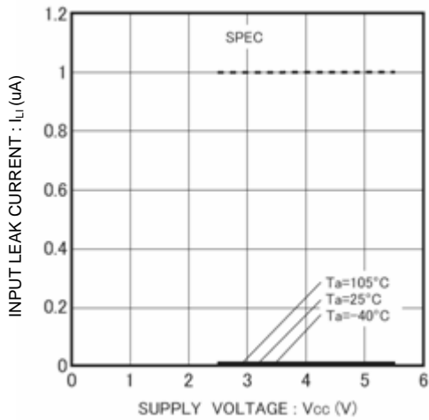
Figure 7. Input leak current I_{ILI} (CS, SK, DI)
