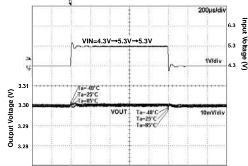
Fig 284. VIN Response
