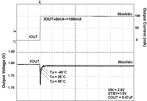
Fig 66. Load Response
