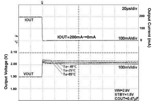
Fig 94. Load Response
