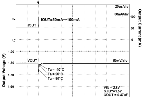
Fig 70. Load Response
