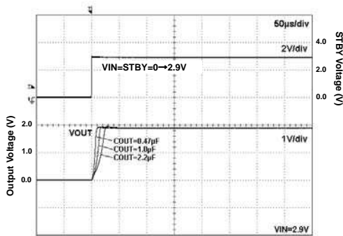
Fig 99. Start Up Time (VIN=STBY) Iout=0mA Iout=0mA
