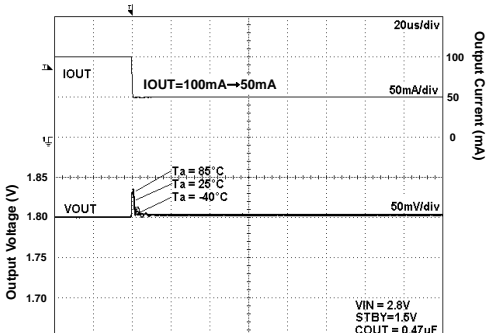
Fig 71. Load Response
