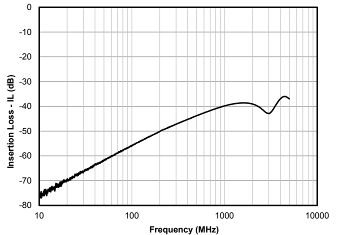
Analog Crosstalk
