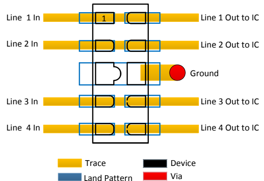
Figure 2 - Trace Routing
