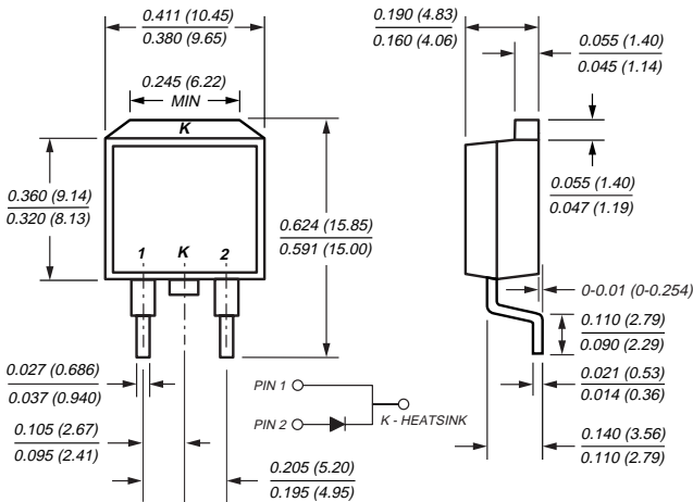
TO-263AB (MBRB10Hxx)
