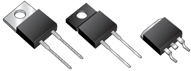
ITO-220AC (MBRF10Hxx)
