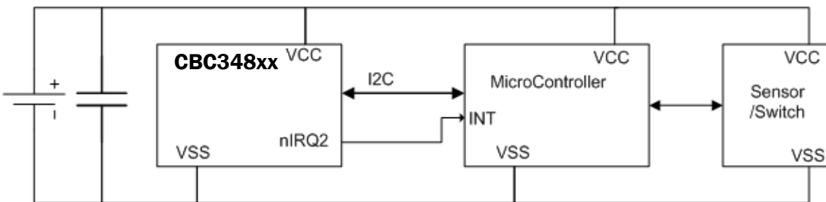
Figure 3: Interrupt-Only Configuration.
