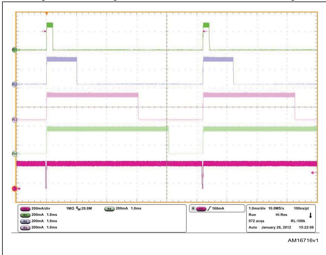
Figure 16. Current regulation - the same channels, different dimming
