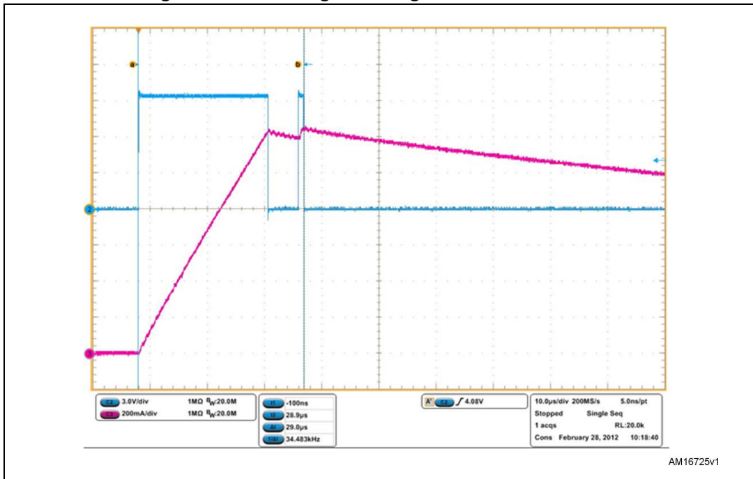
Figure 25. MOSFET gate during short-circuit - 1.065 A
