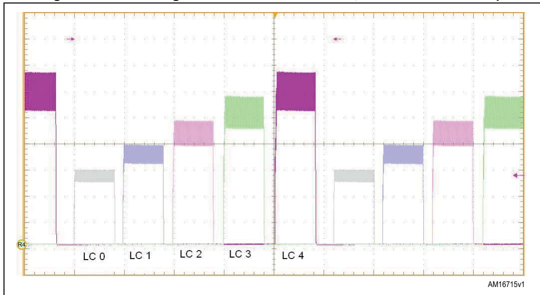
Figure 15. Current regulation - the same channels, different current setup
