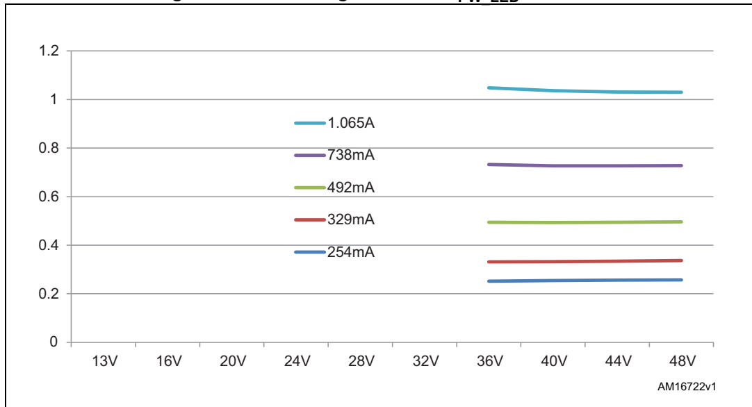
Figure 22. Current regulation vs. V_{PW LED} : 10 LEDs
