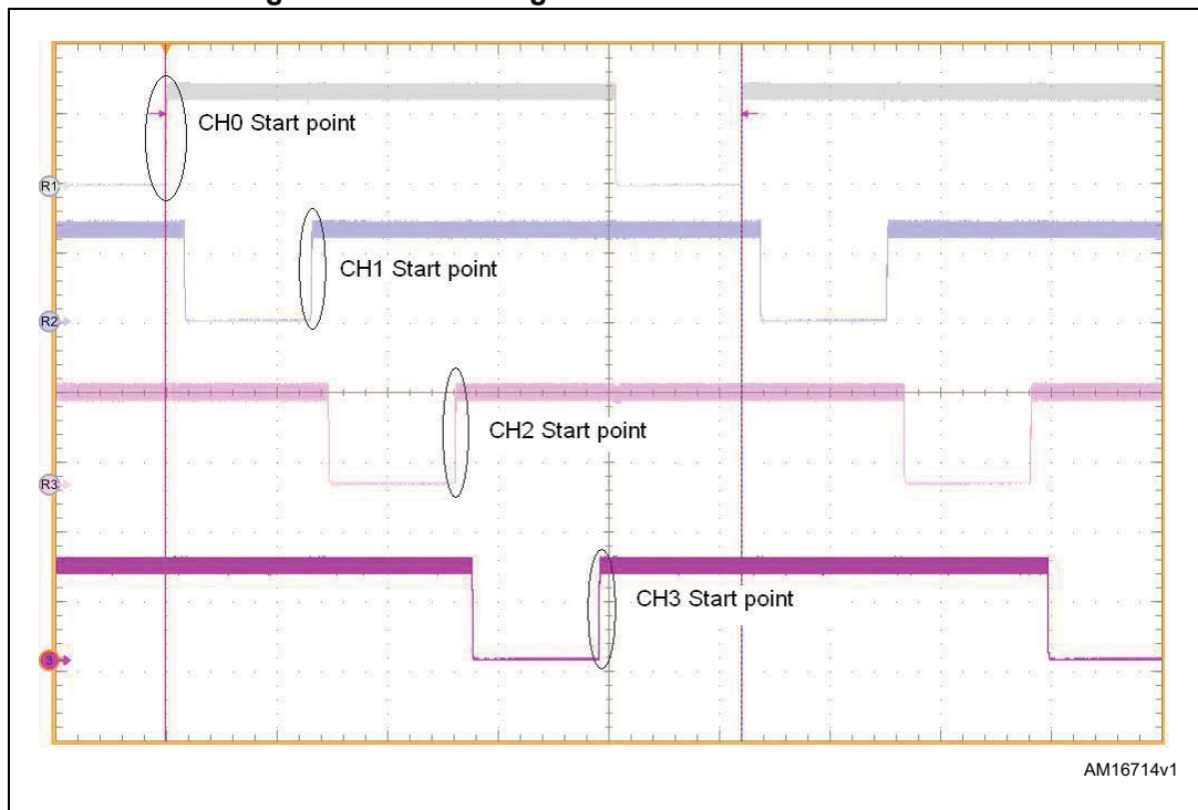
Figure 14. Current regulation - 4 channels at 245 mA
