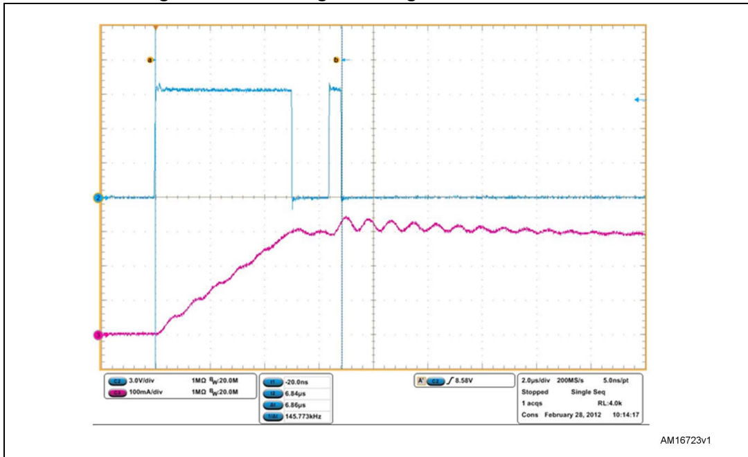
Figure 24. MOSFET gate during short-circuit - 738 mA
