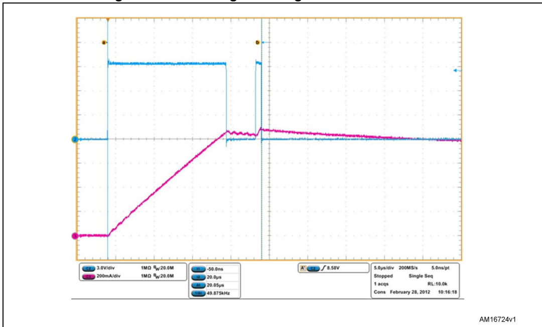
Figure 24. MOSFET gate during short-circuit - 738 mA
