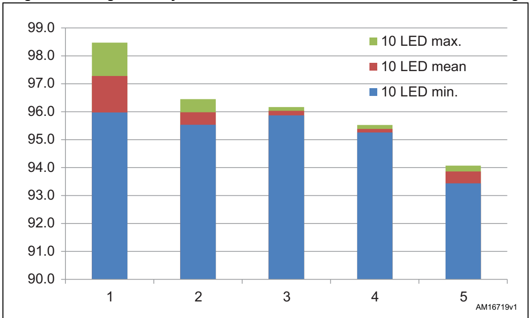
Figure 19. String efficiency based on different current levels - 10 LEDs each string
