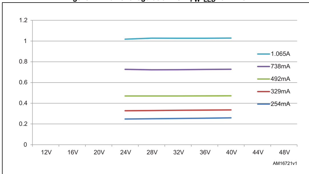
Figure 21. Current regulation vs. V_{PW\_LED} : 6 LEDs
