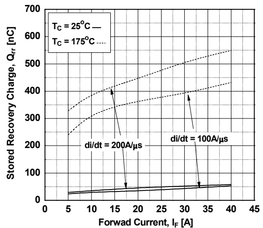
Figure 24. Stored Charge
