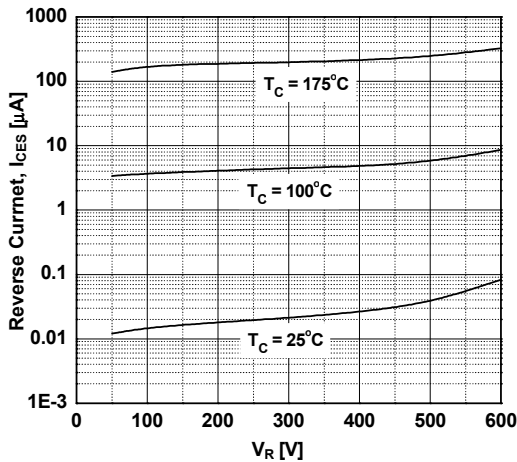
Figure 23. Reverse Current
