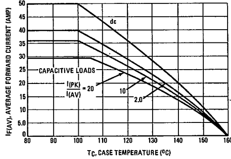
FIGURE 7 - CURRENT DERATING
