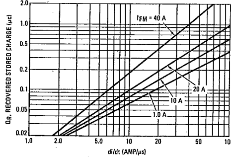
FIGURE 15 - Tj = 150°C
