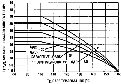
FIGURE 6 - CURRENT DERATING
