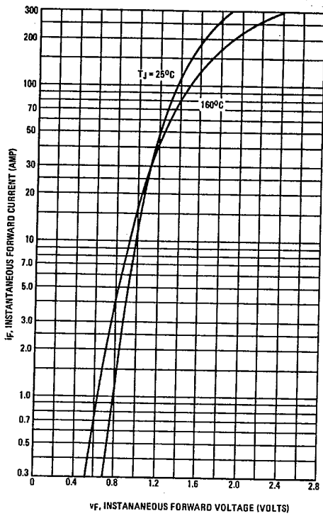
FIGURE 1 - FORWARD VOLTAGE
