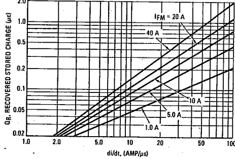
FIGURE 14 - Tj = 100°C
