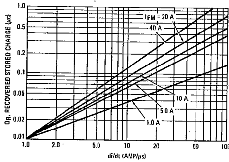
FIGURE 12 - Tj = 25°C
