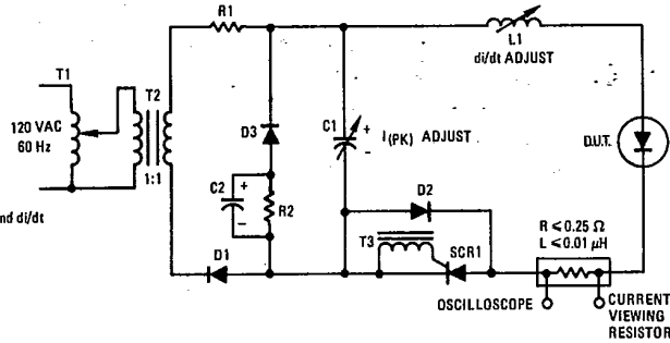
FIGURE 16 — JEDEC REVERSE RECOVERY CIRCUIT
