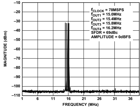
Figure 43. Four-Tone SFDR
