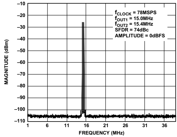
Figure 42. Dual-Tone SFDR
