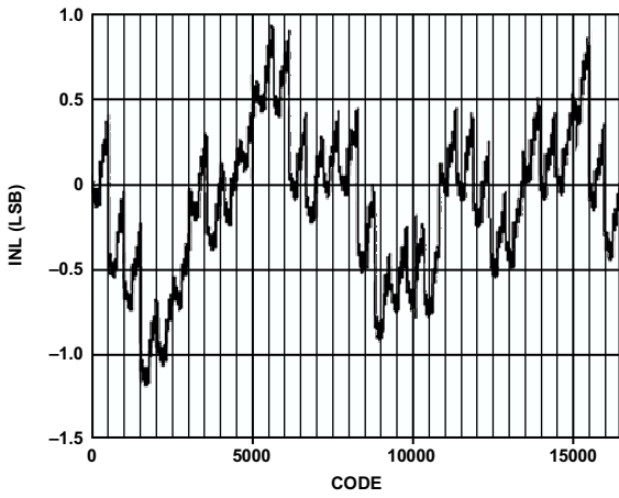
Figure 19. Typical Uncalibrated INL
