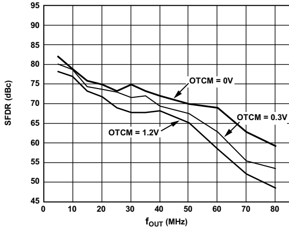
Figure 13. SFDR vs. f_{OUT} and OTCM @ 175 MSPS
