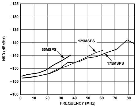
Figure 15. NSD vs. f_{OUT} and f_{CLOCK} @ 0 dBFS
