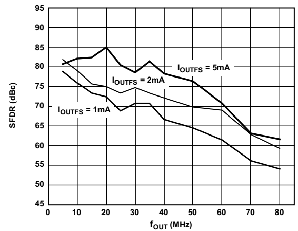
Figure 12. SFDR vs. f_{OUT} and I_{OUTFS} @ 175 MSPS
