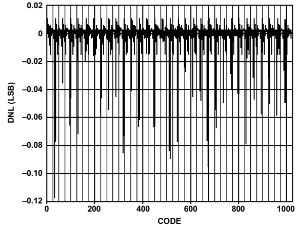
Figure 61. AD9705 Typical Uncalibrated DNL
