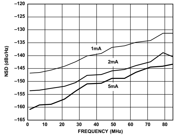
Figure 16. NSD vs. f_{OUT} and I_{OUTS} @ 175 MSPS
