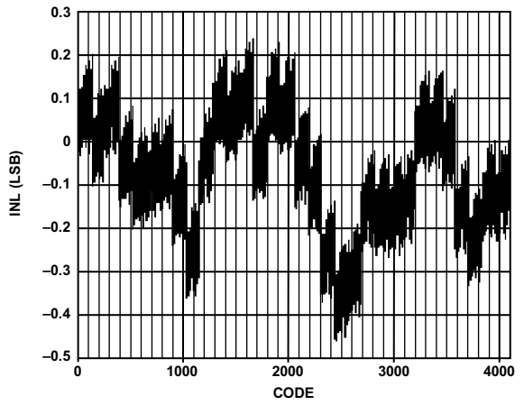
Figure 62. AD9706 Typical Uncalibrated INL
