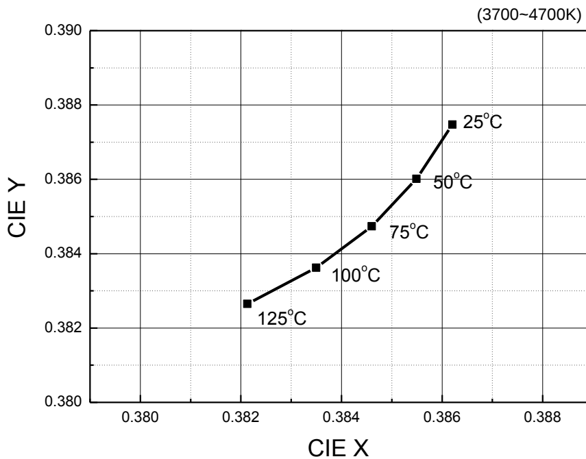
Fig 8. Chromaticity Coordinate vs. Junction Temperature, I_F=40\text{mA}
