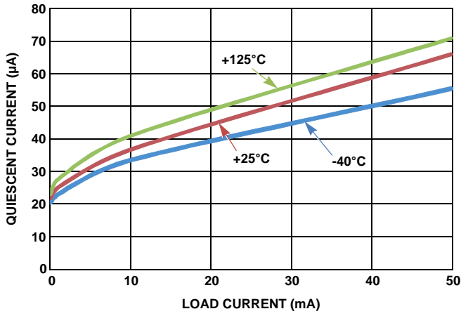
FIGURE 3. QUIESCIENT CURRENT vs LOAD CURRENT
