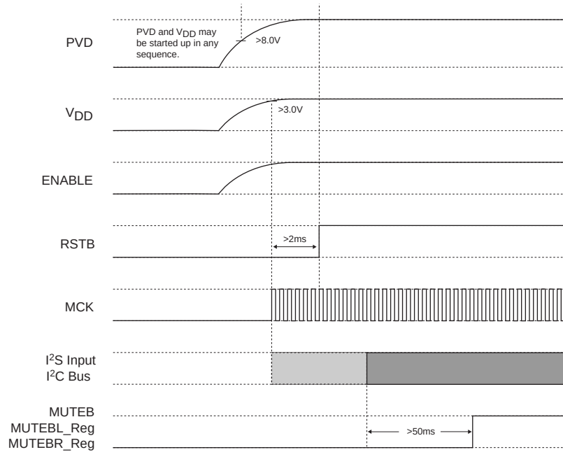
Figure 3.1 Start sequence
