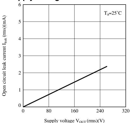
Fig.8 Open Circuit Leak Current vs. Supply Voltage
