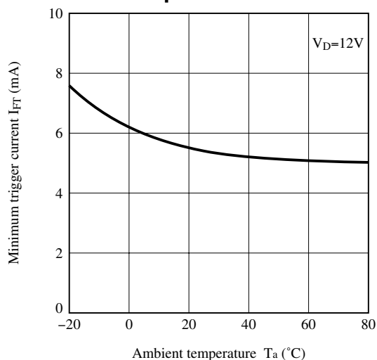
Fig.6 Minimum Trigger Current vs. Ambient Temperature
