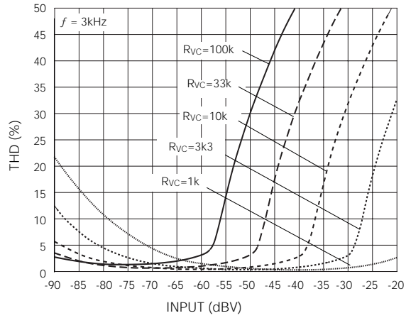
Fig. 8 Distortion vs Input
