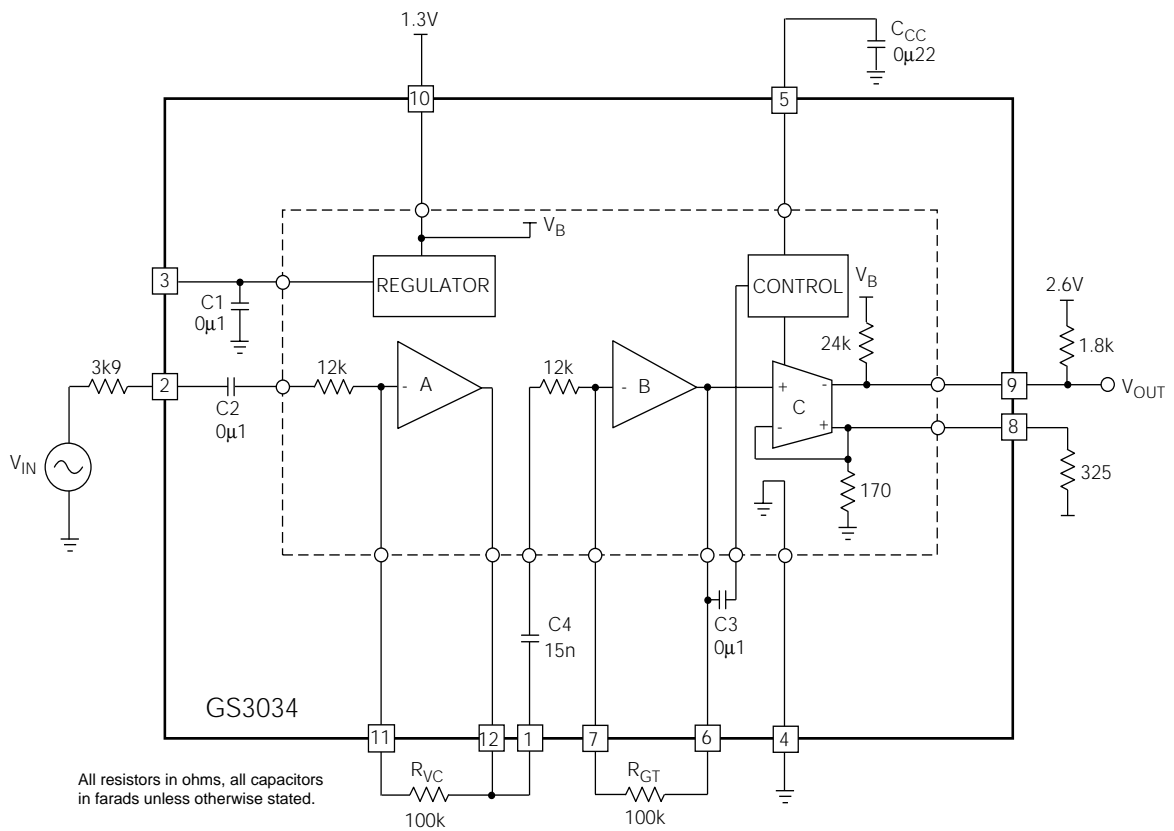
Fig. 4 Characterization Circuit
