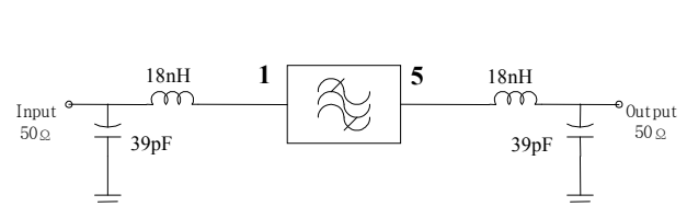
Matching Schematic
