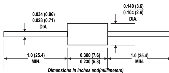
DO-204AC (DO-15)
