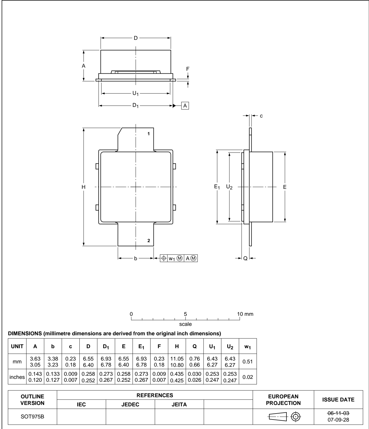
Fig 5. Package outline SOT975B
