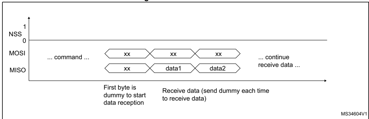
Figure 5. Read data frame
