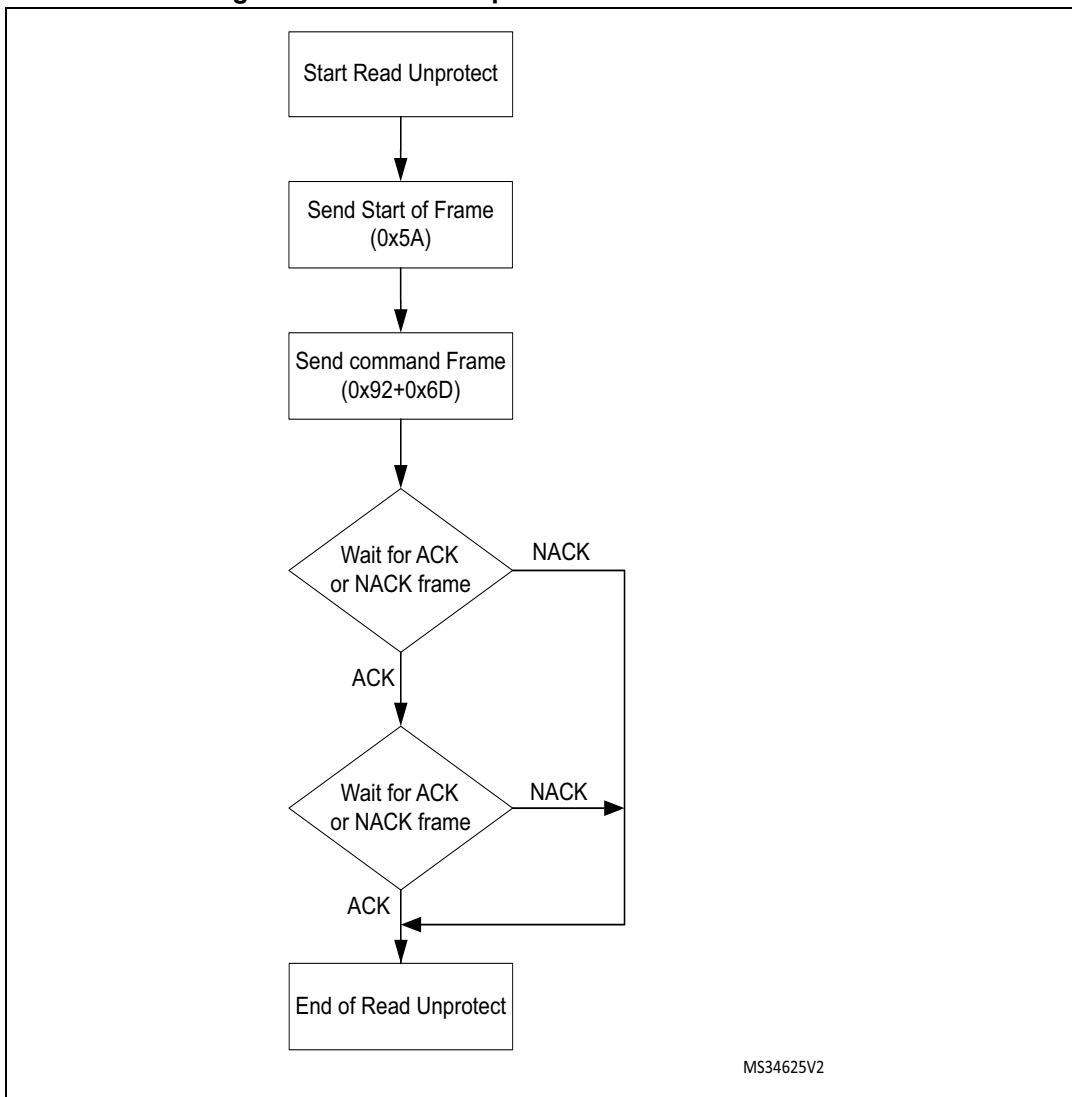
Figure 26. Readout Unprotect command: master side
