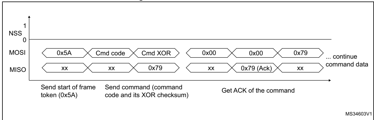
Figure 4. SPI command frame
