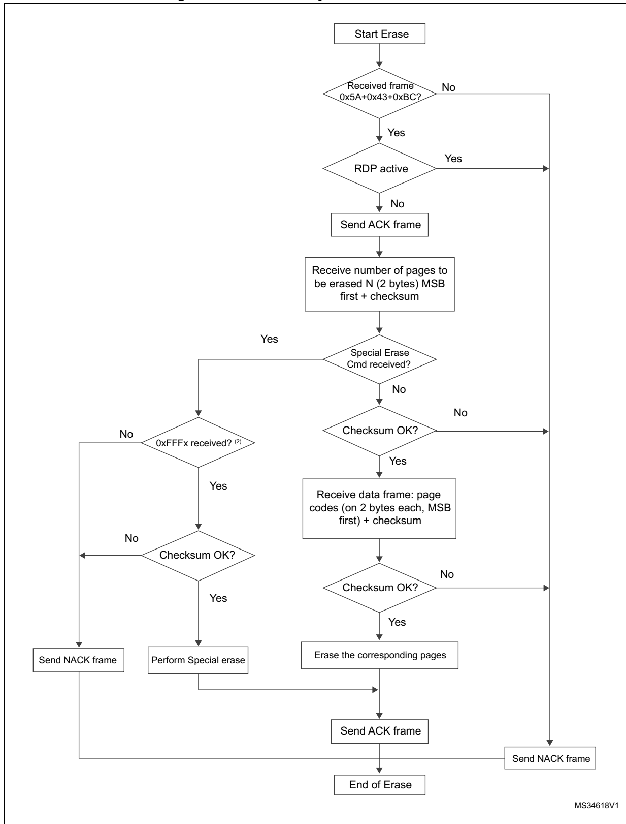
Figure 19. Erase Memory command: slave side
