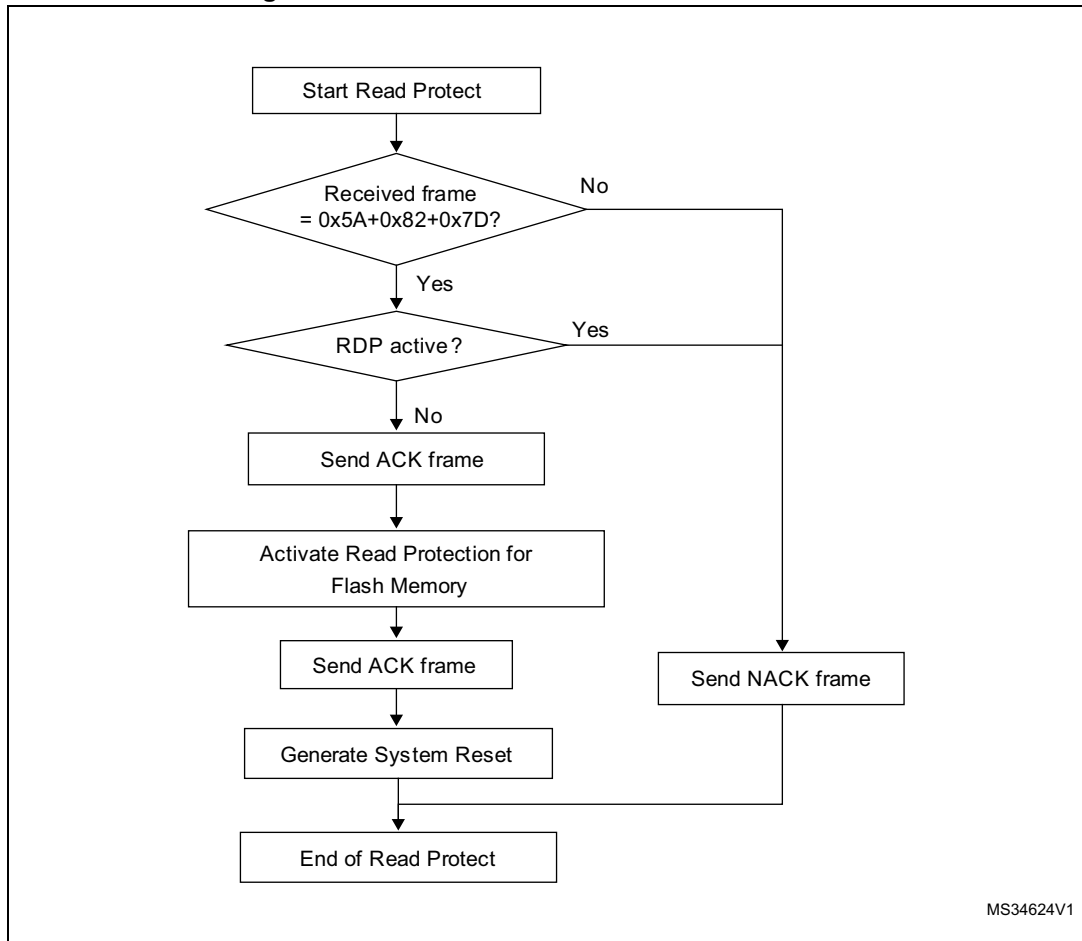
Figure 25. Readout Protect command: slave side
