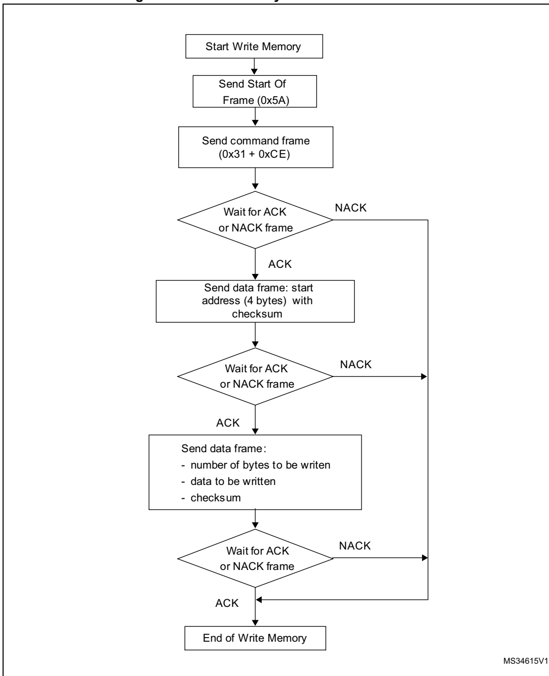
Figure 16. Write Memory command: master side
