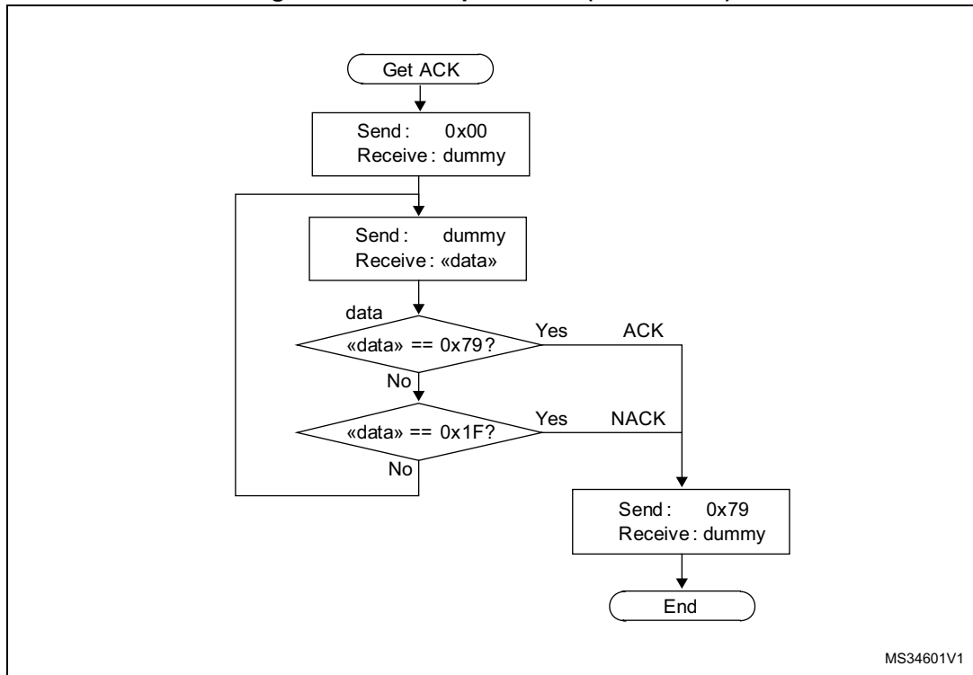
Figure 2. Get ACK procedure (Master side)
