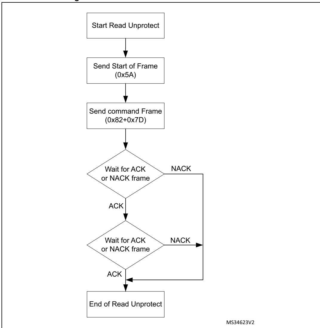
Figure 24. Readout Protect command: master side
