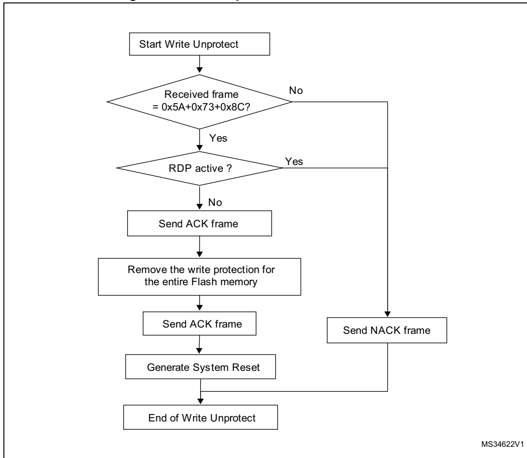
Figure 23. Write Unprotect command: slave side
