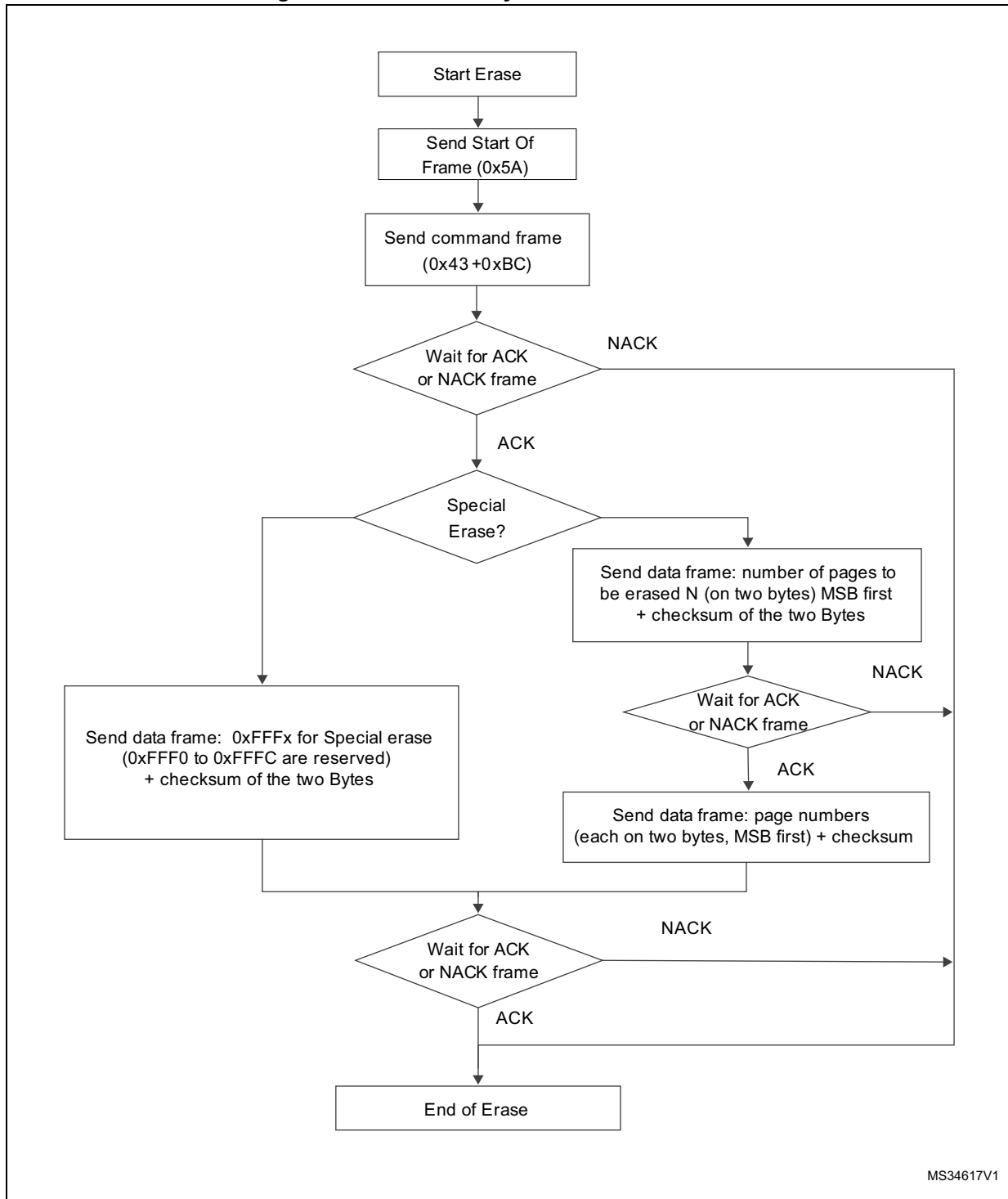
Figure 18. Erase Memory command: master side
