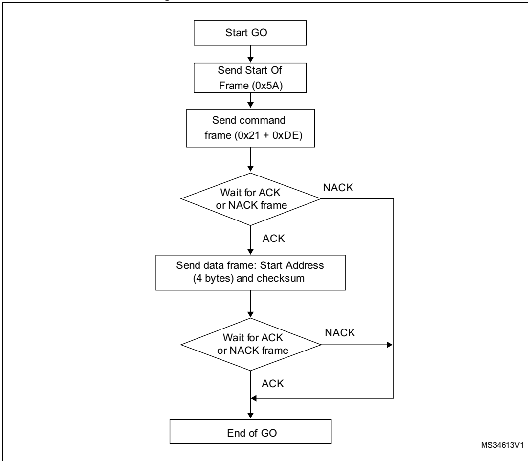
Figure 14. Go command: master side
