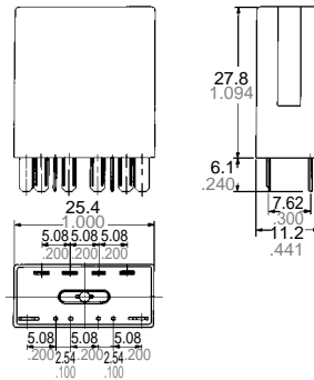
Amber sealed type
