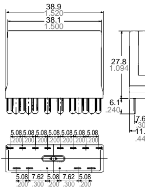
Amber sealed type
