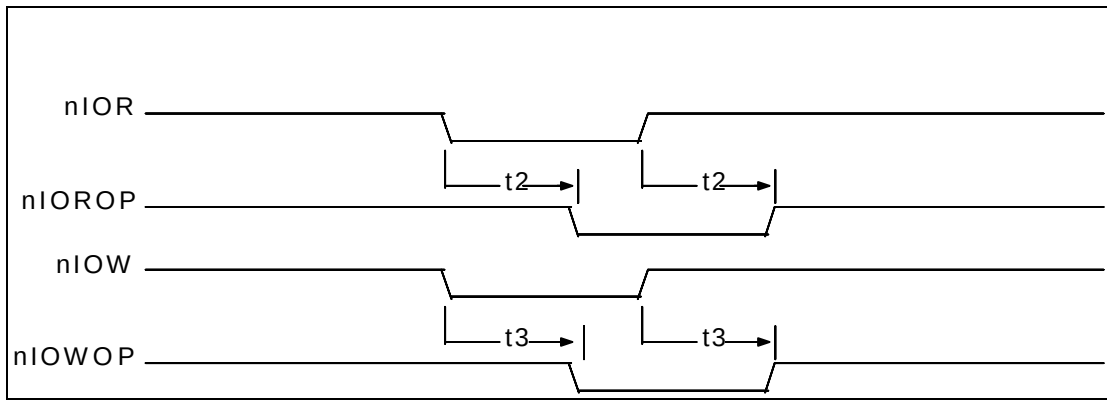
FIGURE 23 - nIOROP, nLOWOP TIMING
