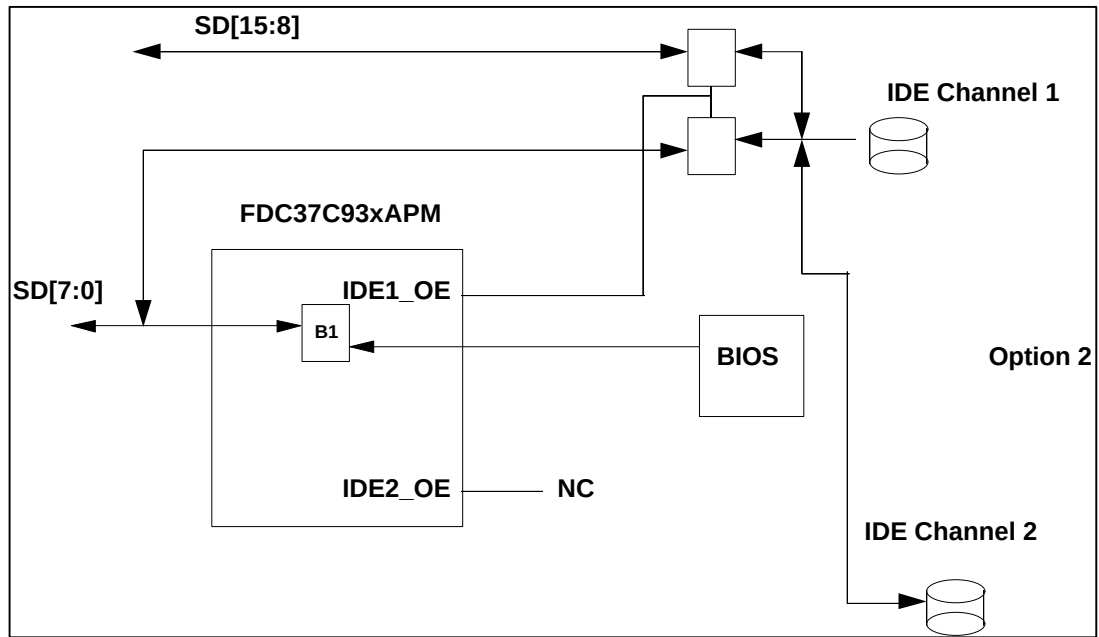
FIGURE 3 - IDE OUTPUT ENABLE OPTION 2
