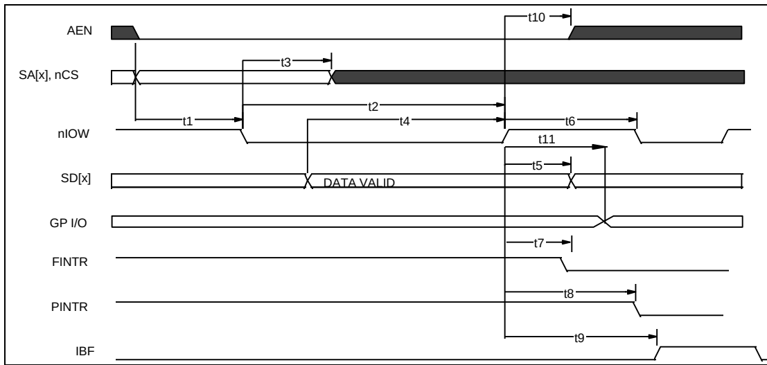
FIGURE 18 - ISA WRITE
