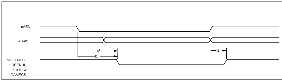
FIGURE 28 - IDE INTERFACE TIMING
