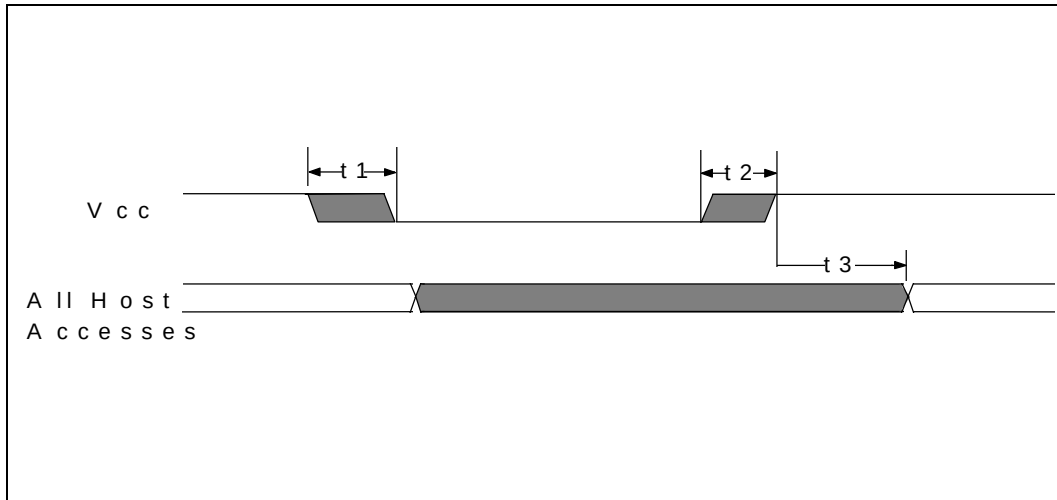
FIGURE 17 - POWER-UP TIMING
