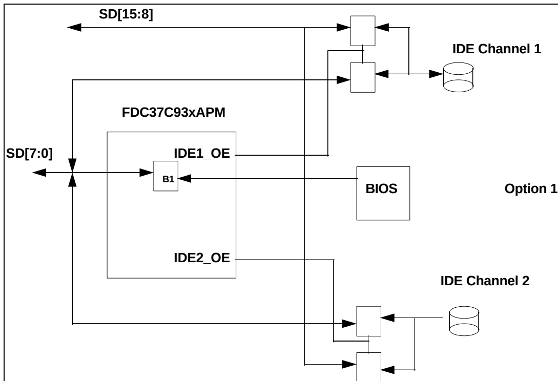
FIGURE 2 - IDE OUTPUT ENABLE OPTION 1
