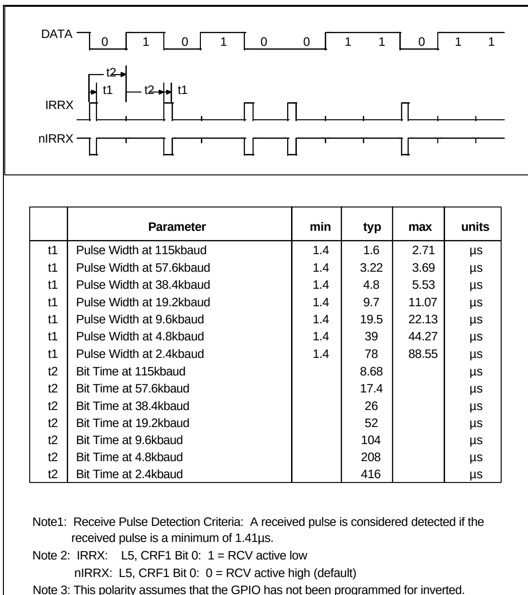
FIGURE 38 - IrDA RECEIVE TIMING
