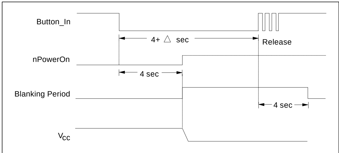
FIGURE 12 - BLANKING PERIOD
