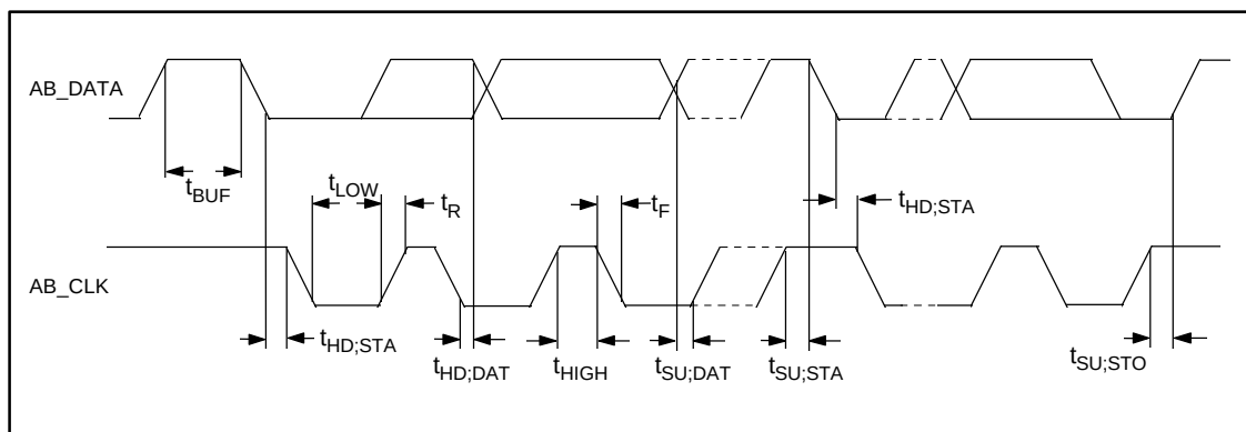
FIGURE 37 - ACCESS.BUS TIMING
