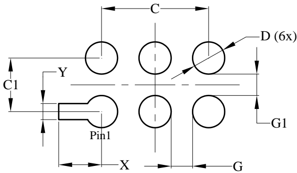
(4) X2-DFN1409-6
