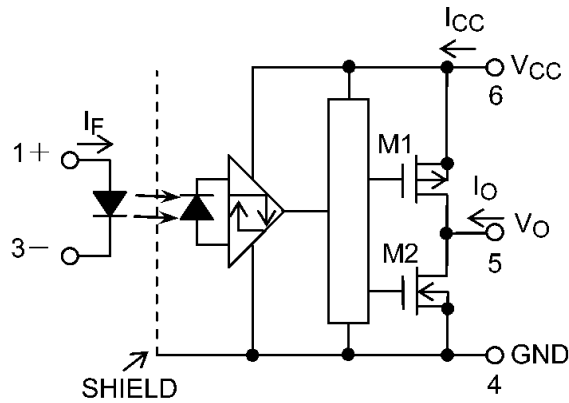
Fig. 5.1 Internal Circuit
