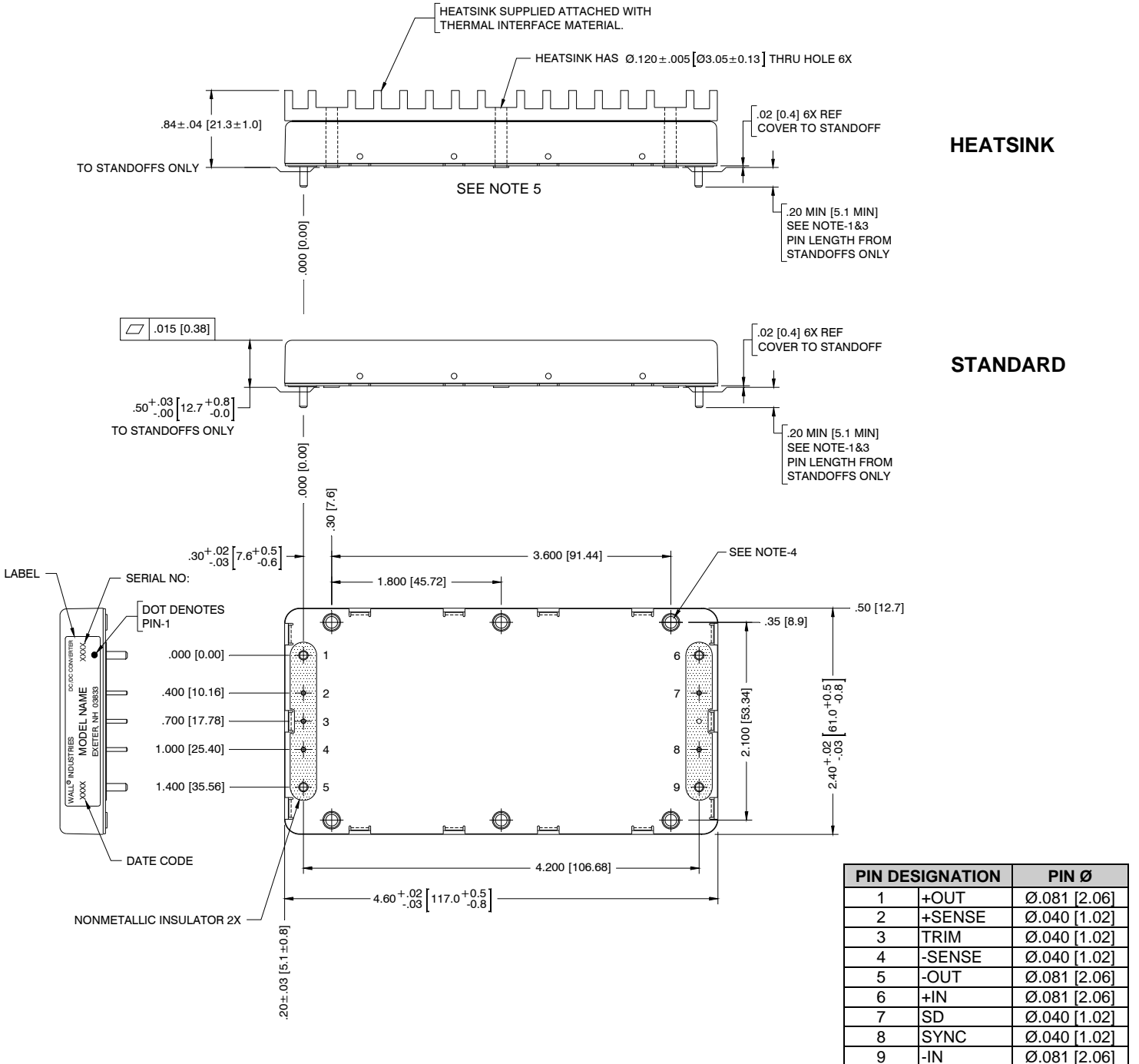
Figure 1: Mechanical Dimensions
