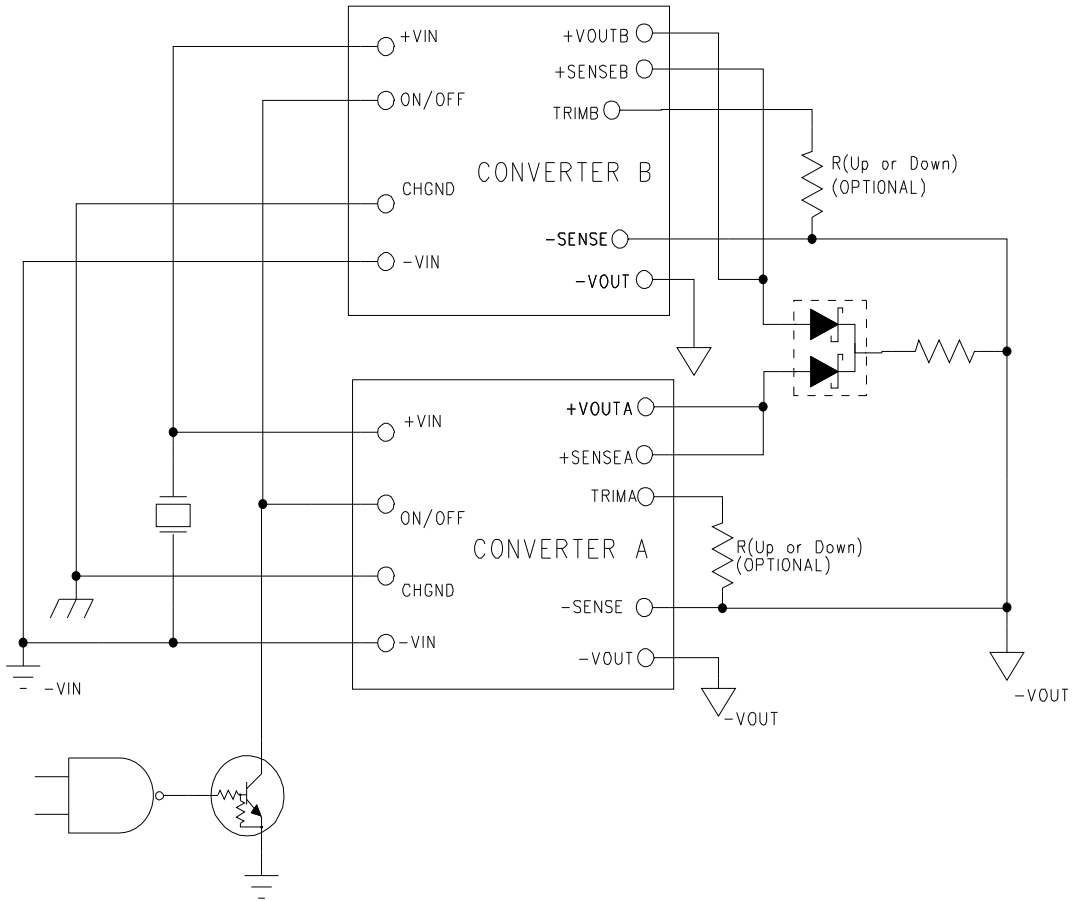
Figure 9: Paralleling Converters
