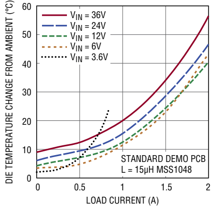
Die Temperature Rise vs Load Current, V_{OUT} = 5V , f_{SW} = 750\text{kHz}
