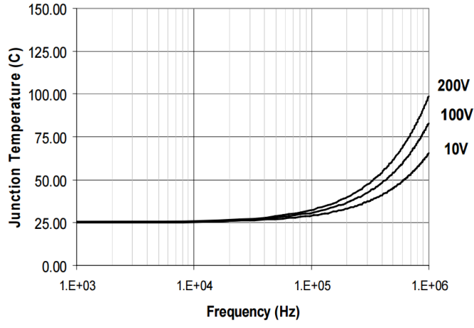
Figure 30. IR2010 Tj vs. Frequency R_{GATE} = 22\Omega , V_{CC} = 15V with IRFBC30
