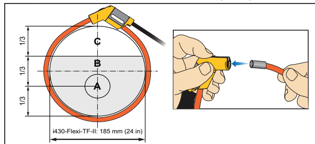
Figure 1. Connecting the flexible probe around the conductor.
