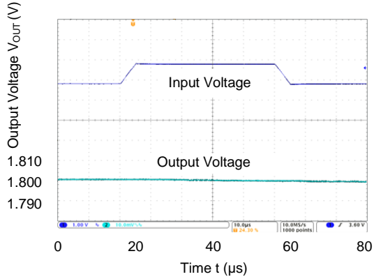
Line Transient Response Waveforms V_{OUT}=1.8V
