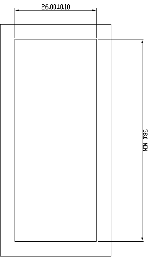
BEZEL CUT-OUT CENTER SPACING DETAIL BEZEL THICKNESS:0.8-2.6
