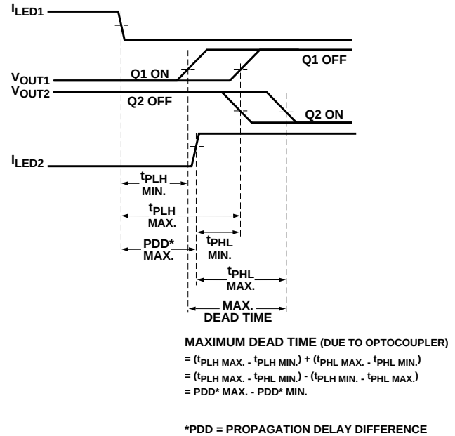
Figure 30. Waveforms for Dead Time Calculation.
