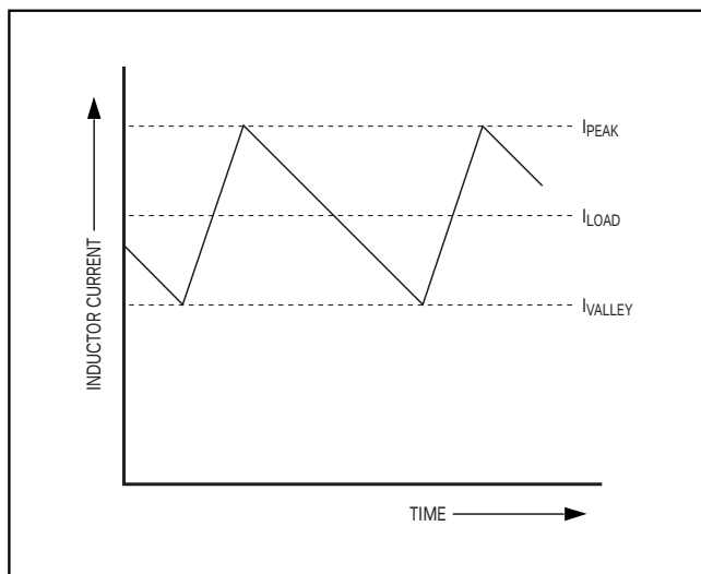
Figure 4. Inductor-Current Waveform
