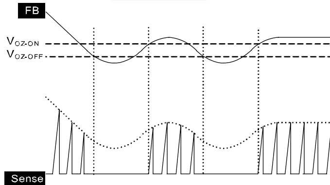
Figure 11. Burst-Mode Diagram
