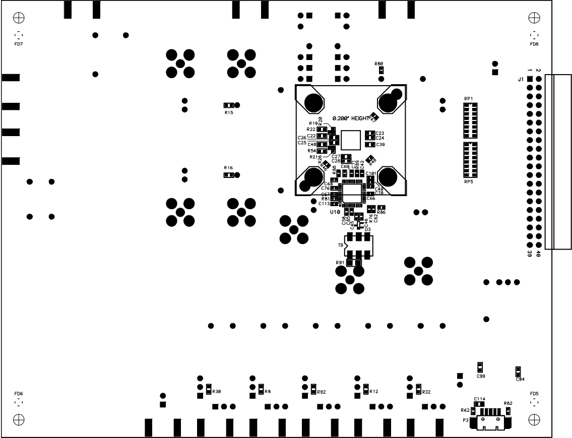
Figure 122. Assembly—Secondary Side
