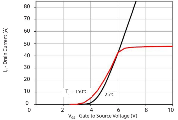
Transfer Characteristics
